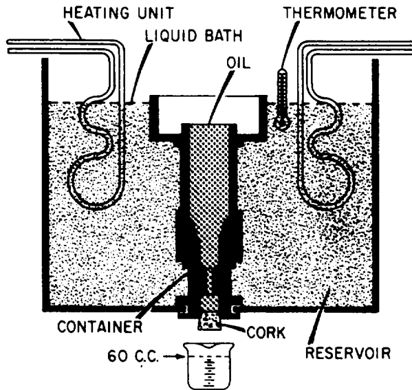
Figure 3-1.—Saybolt viscometer.
